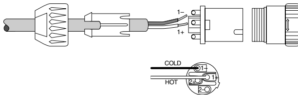
Speakon Connectors
