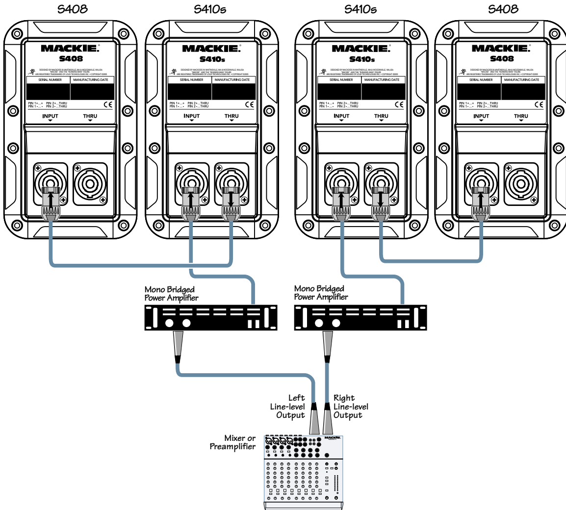
S410s AND S408: WITH A MIXER AND TWO POWER AMPLIFIERS
